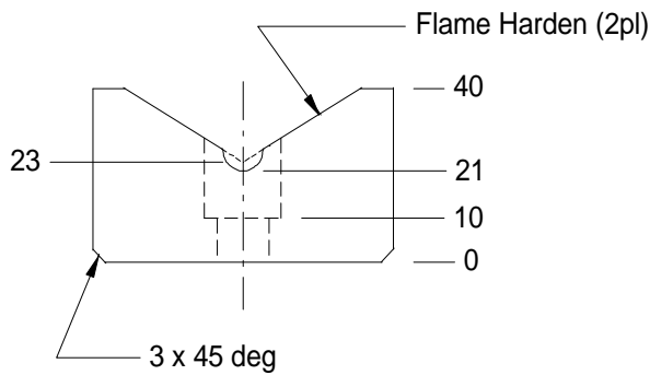
U-Block Profile
