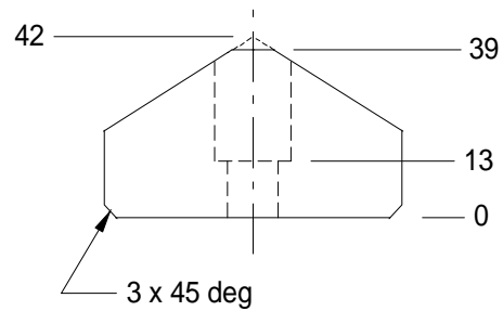
V-Block Profile
